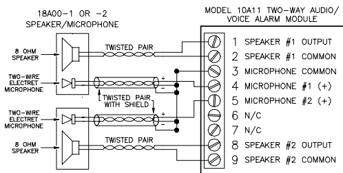
Figure 1 - Speaker/Microphone Connections
